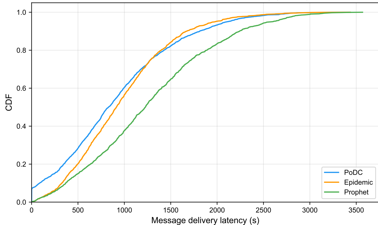
Cumulative distribution of delivery latency (N=100)
