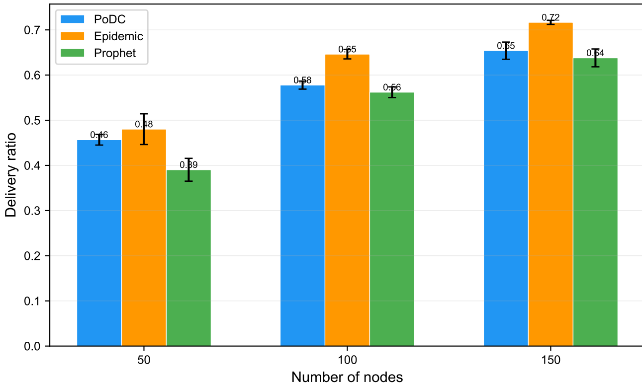
Delivery ratio by protocol and network size
