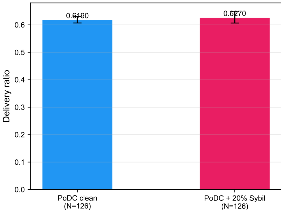
Sybil attack impact on delivery ratio
