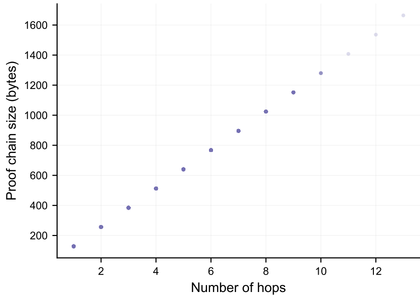
Proof size vs. hop count
