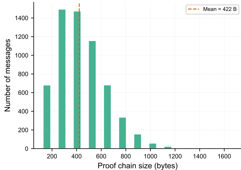
Distribution of proof sizes
