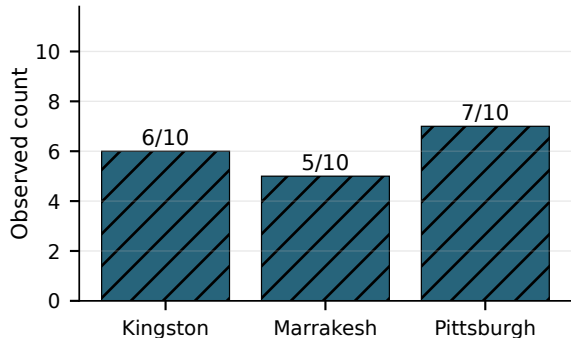
Stable trajectories
