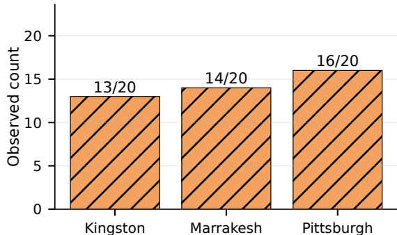
Aligned steps
