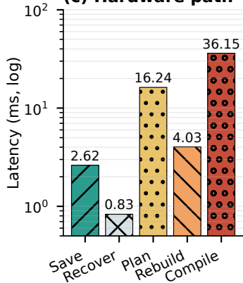
(c) Hardware path
