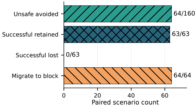
(b) Paired change: \tau = .05 vs .15
