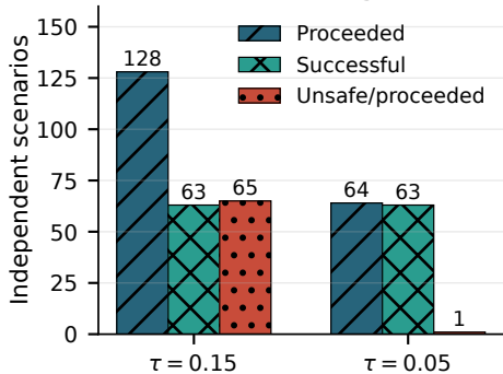
(a) Fresh operating points
