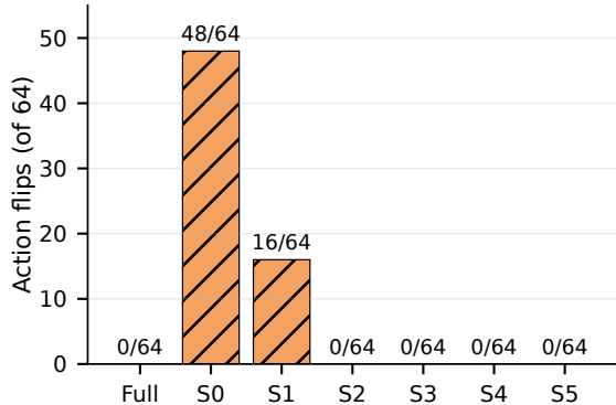
(b) Decision agreement
