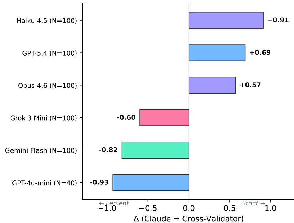
(b) Bias Direction Across Models
