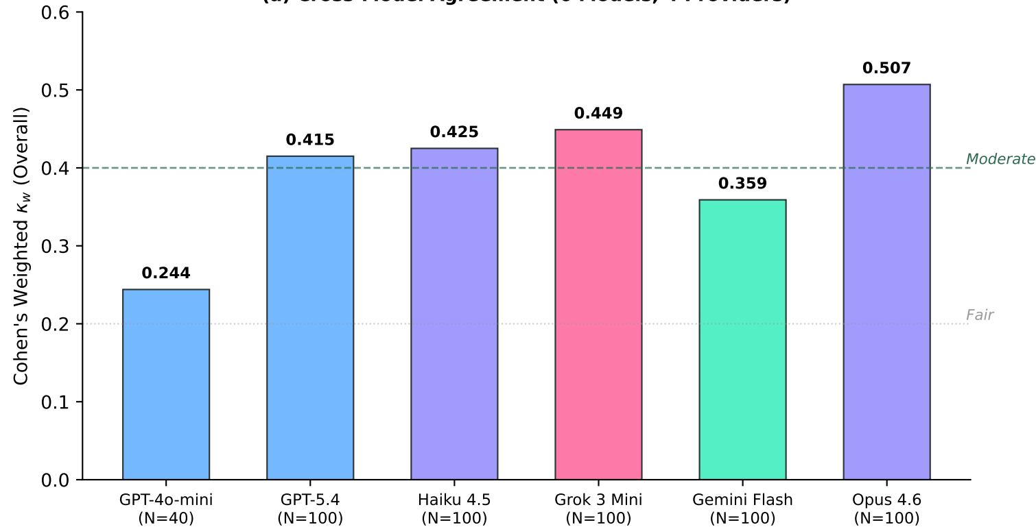
(a) Cross-Model Agreement (6 Models, 4 Providers)
