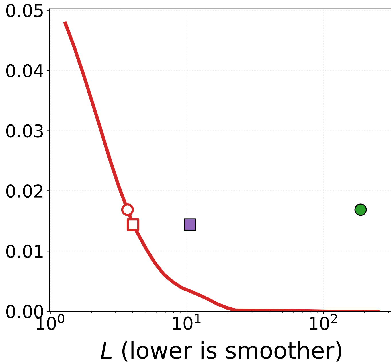
NeurIPS
