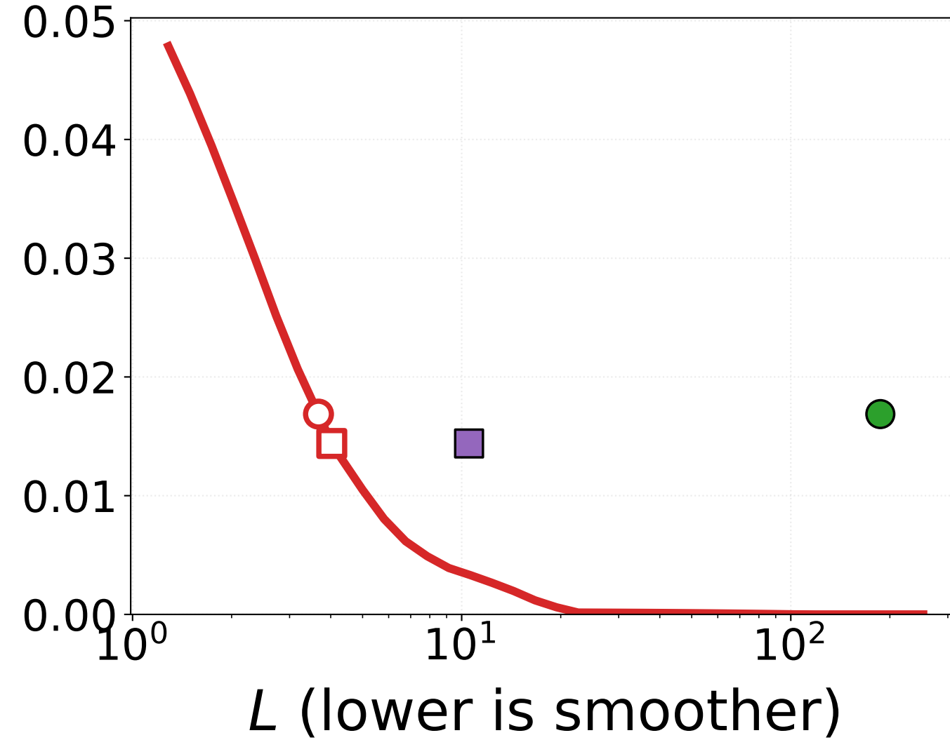
NeurIPS
