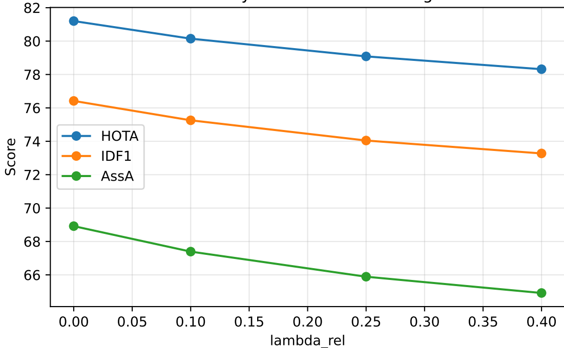
Sensitivity to Relation Prior Weight
