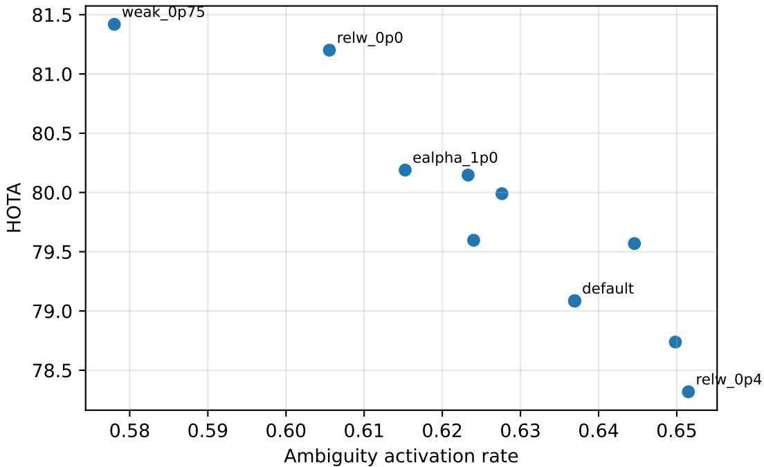
Effect of Ambiguity Gating Selectivity
