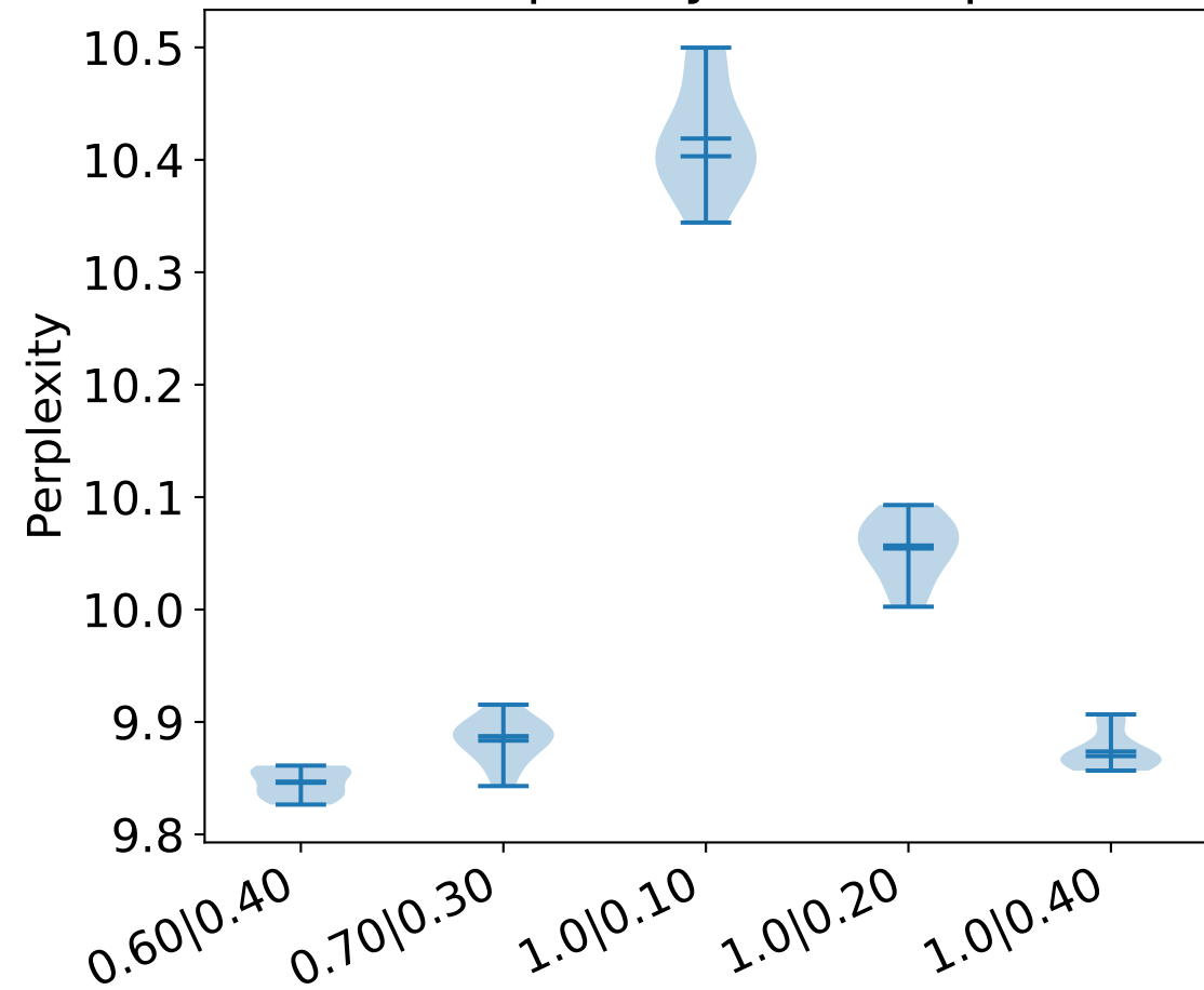
Token-Sparsity Action-Space
