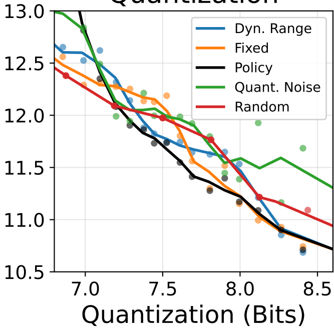
Quantization
