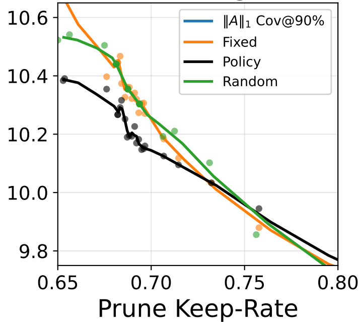
Pruning
