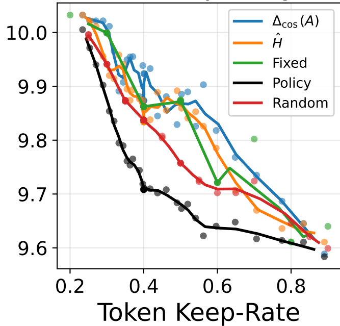
Token Sparsity
