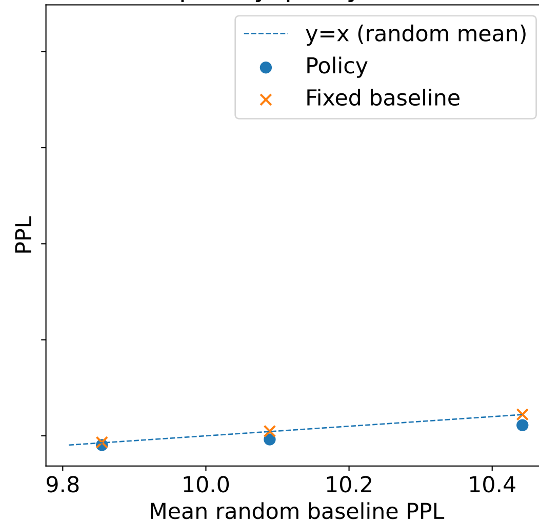
Token sparsity: policy vs random
