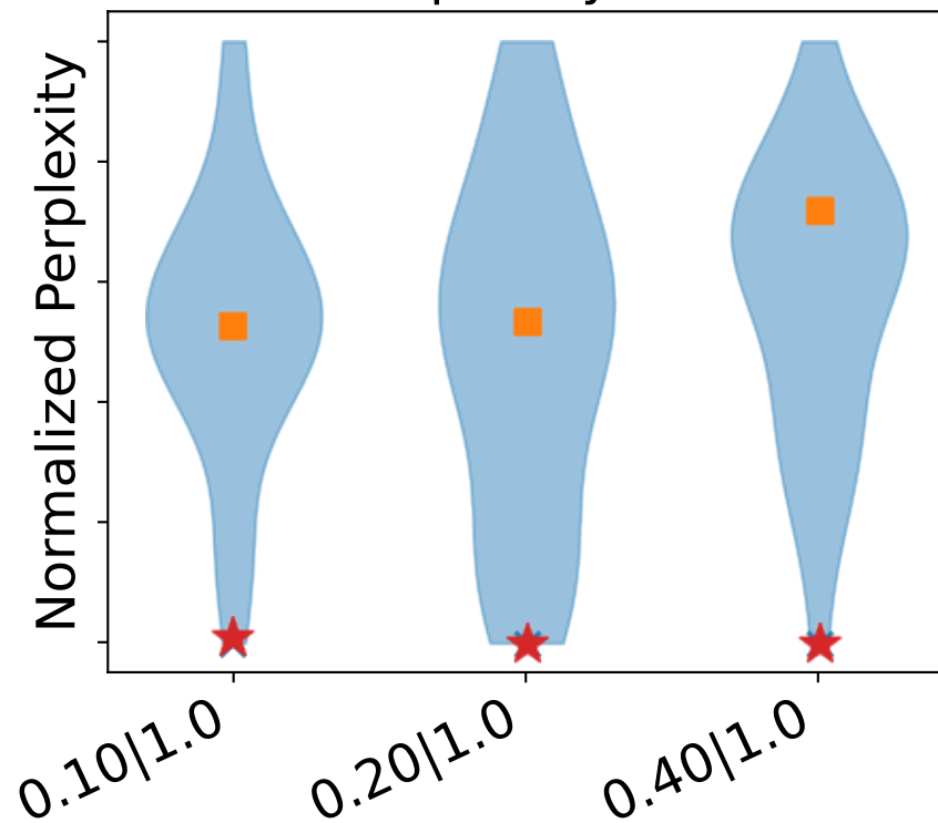
Token-Sparsity Policies
