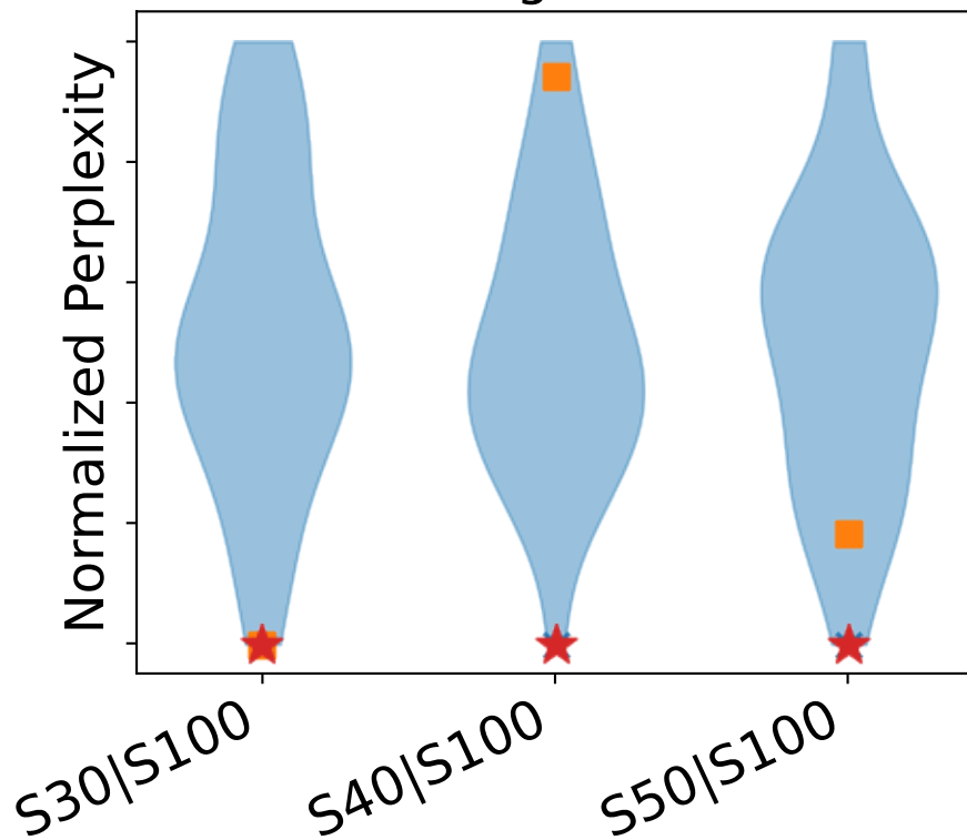
Pruning Policies
