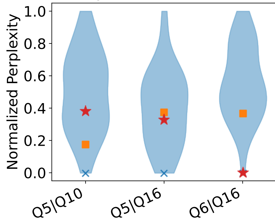
Quantization Policies
