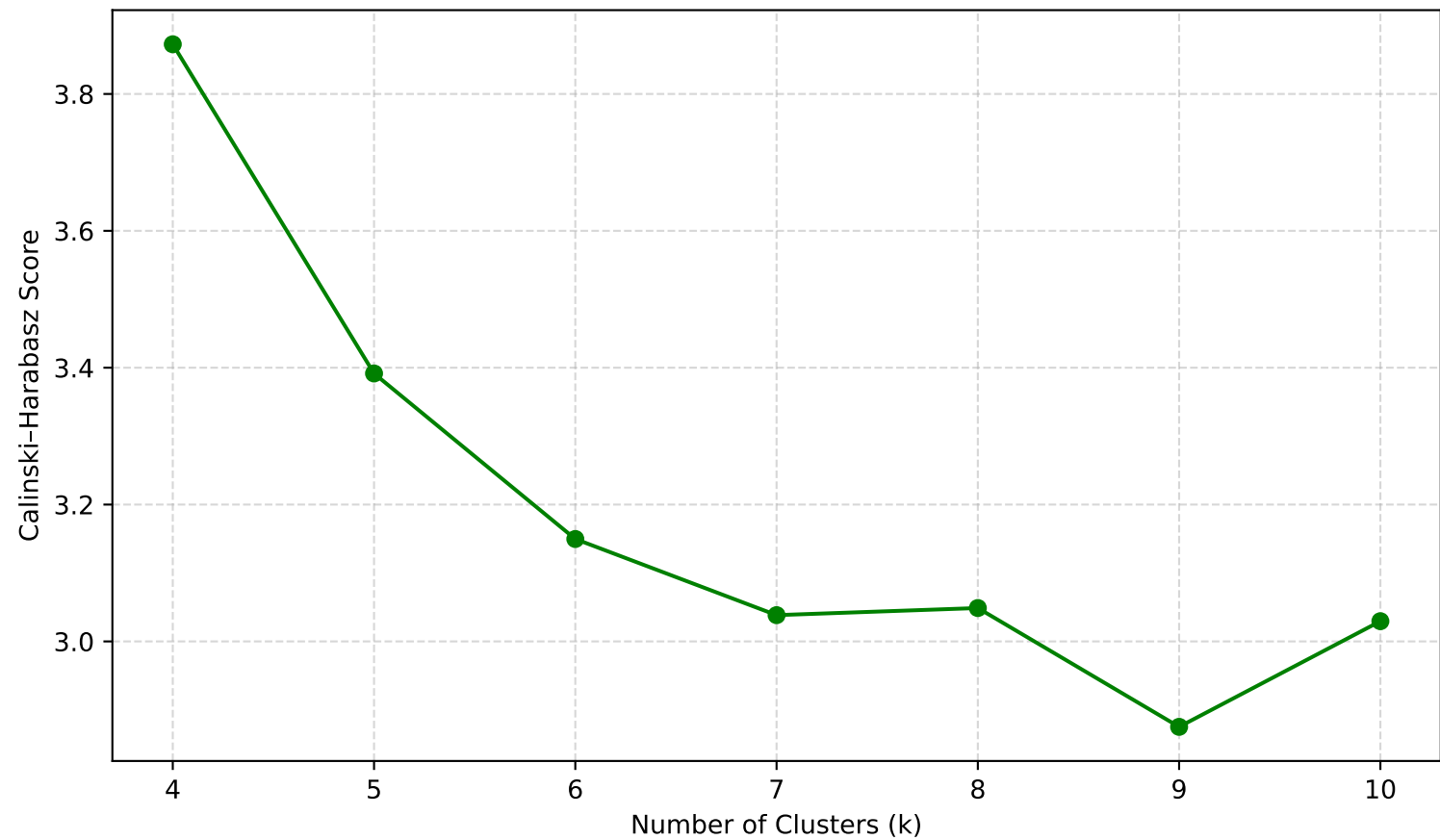
CH Score vs. k
