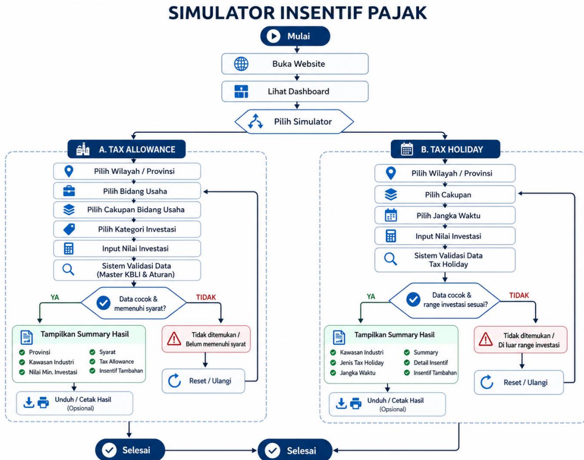
Gambar 3. Flowchart alur fitur website simulator insentif pajak
