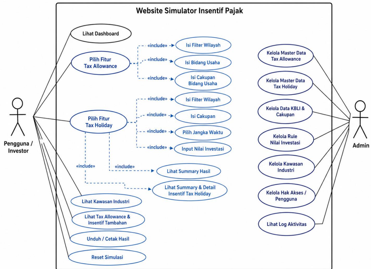
Gambar 2. Diagram use case website simulator insentif pajak
