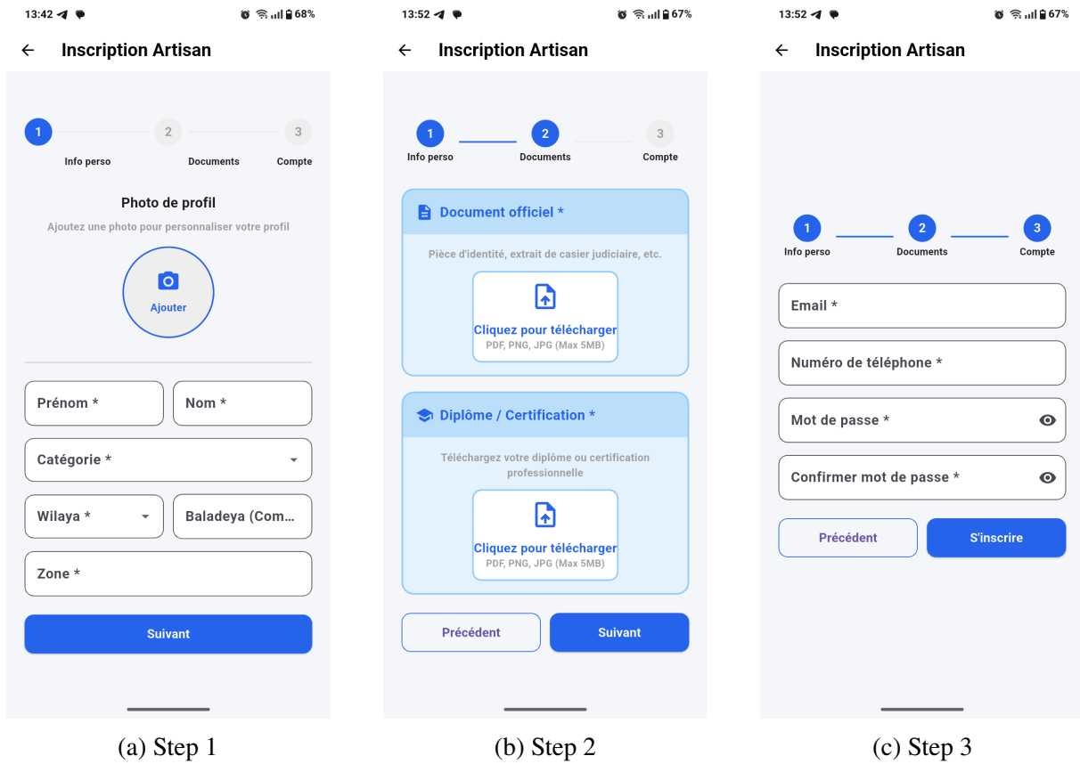
Figure 3.10: Create Artisan Account Interface
