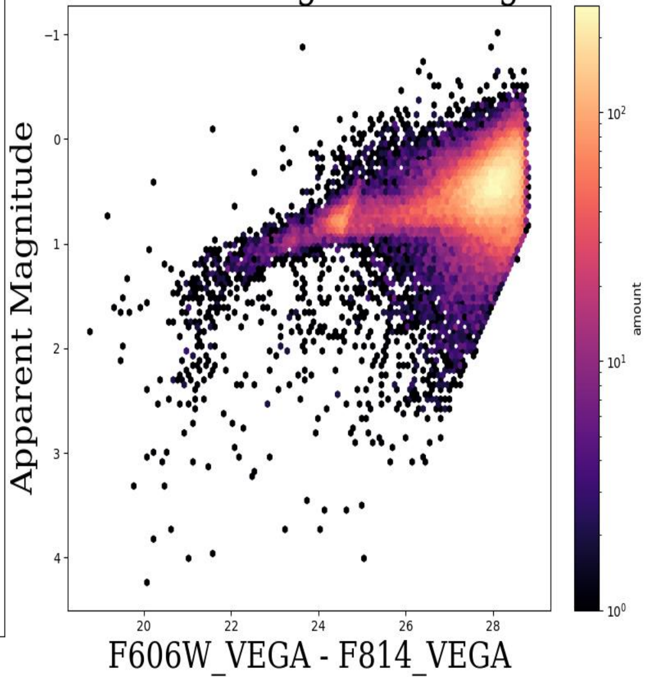
N205 Color Magnitude Diagram
