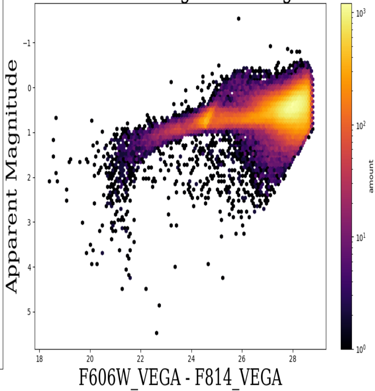
ANDIV Color Magnitude Diagram
