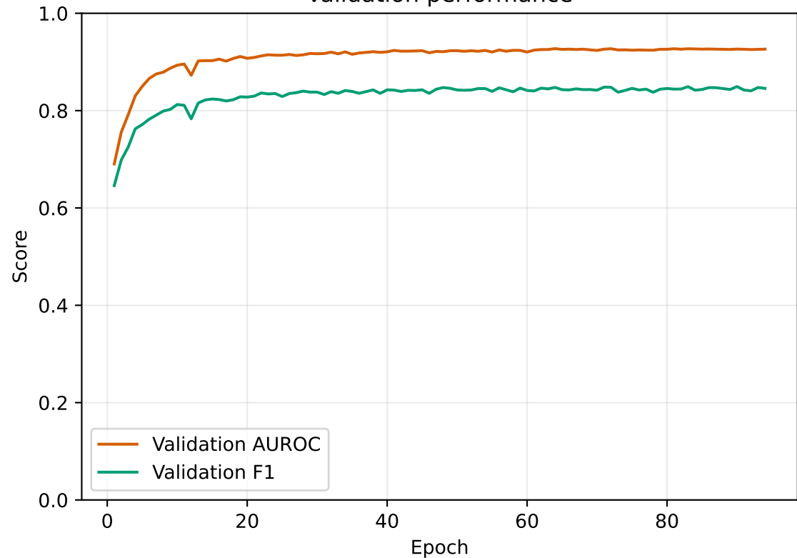
Validation performance
