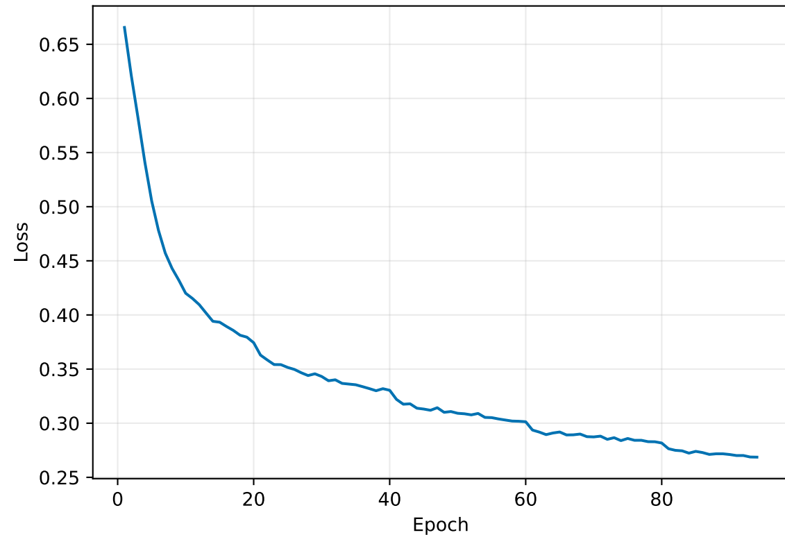
Training loss
