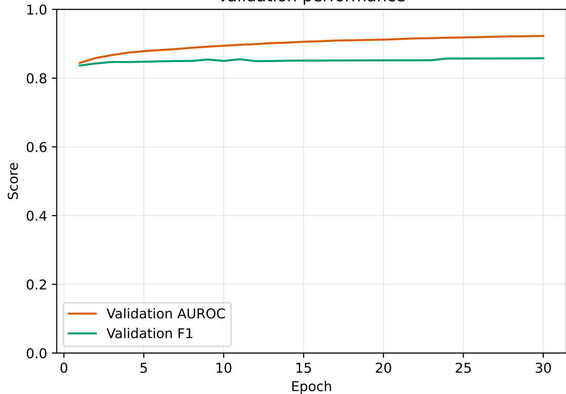
Validation performance
