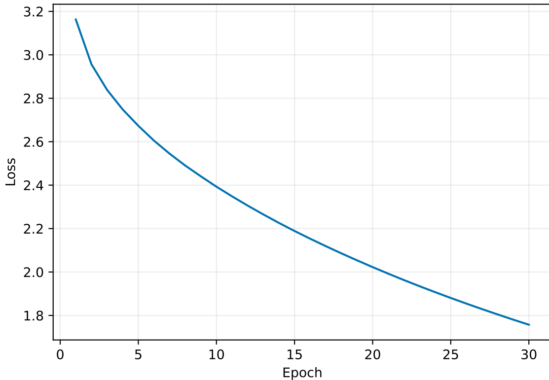
Training loss
