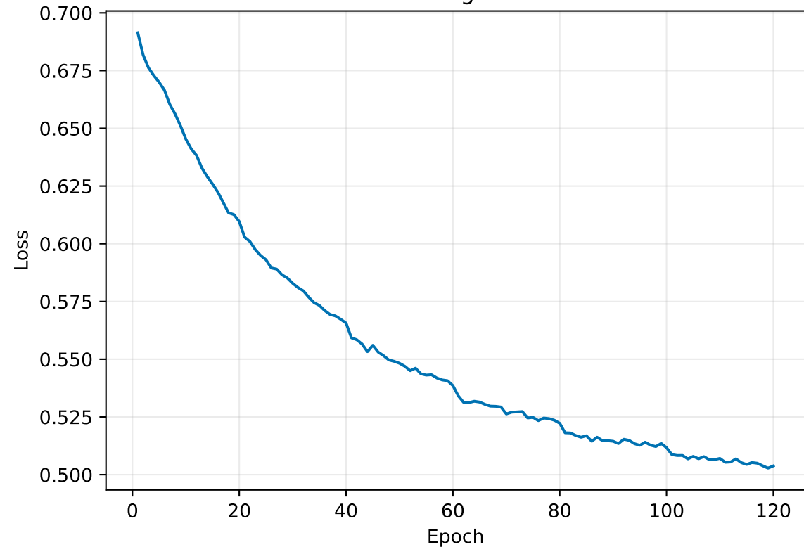
Training loss
