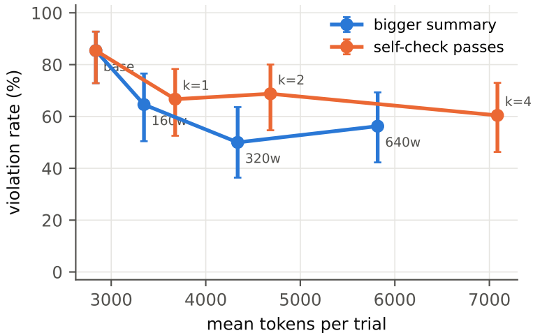
Idea 1 regraded: retention vs. repair per token
