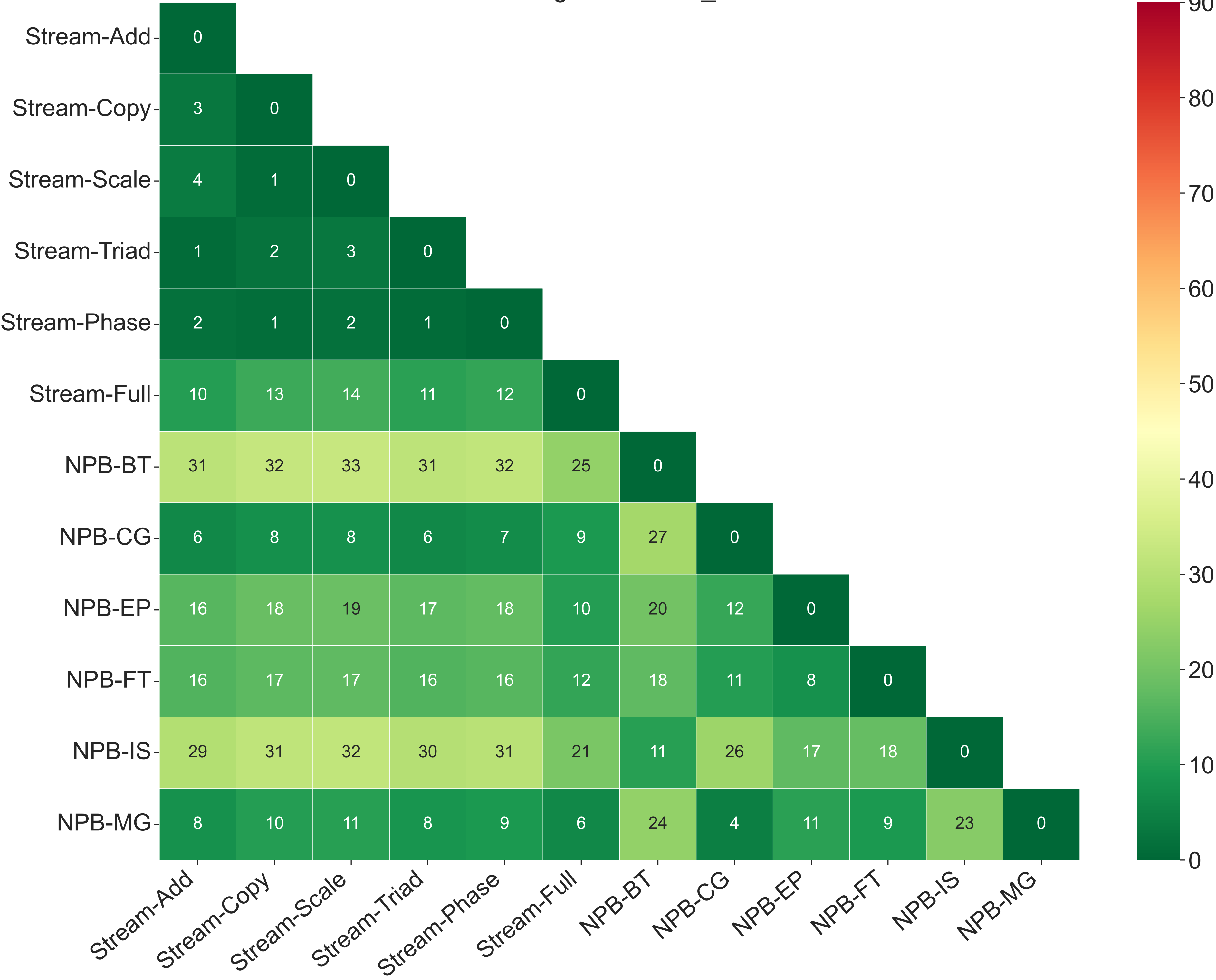
JS-divergence PCAP_124.0
