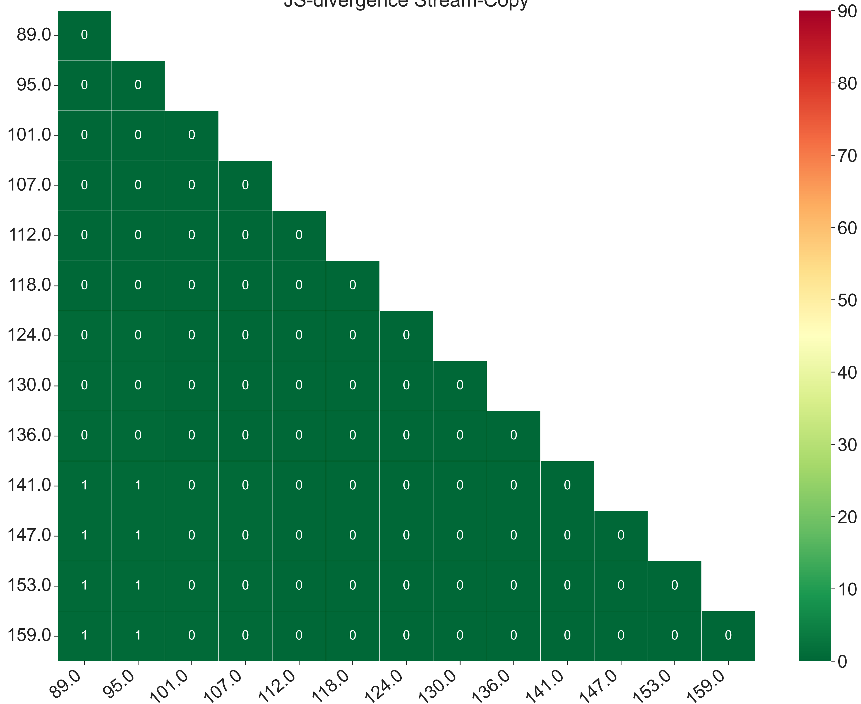
JS-divergence Stream-Copy
