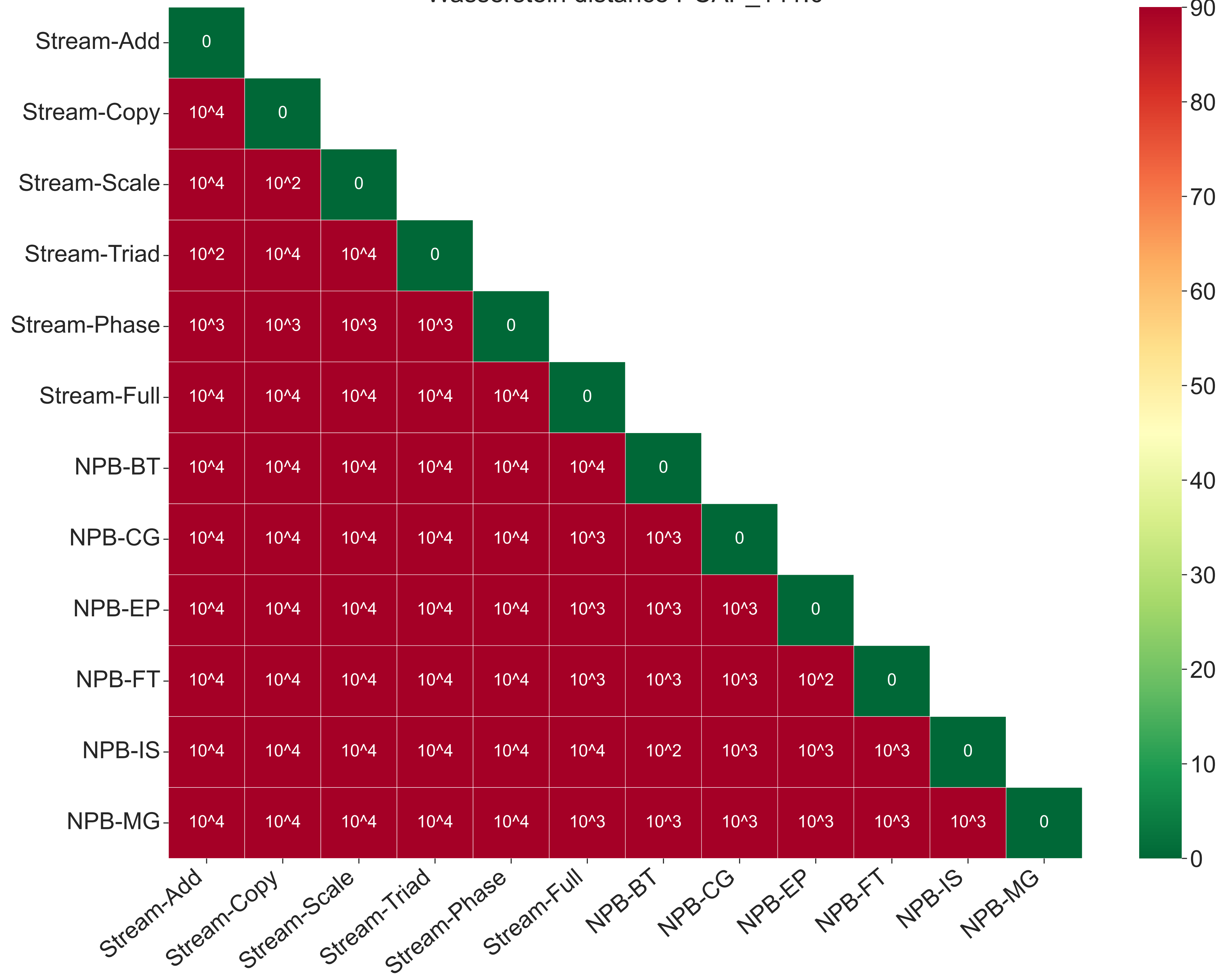
Wasserstein distance PCAP_141.0
