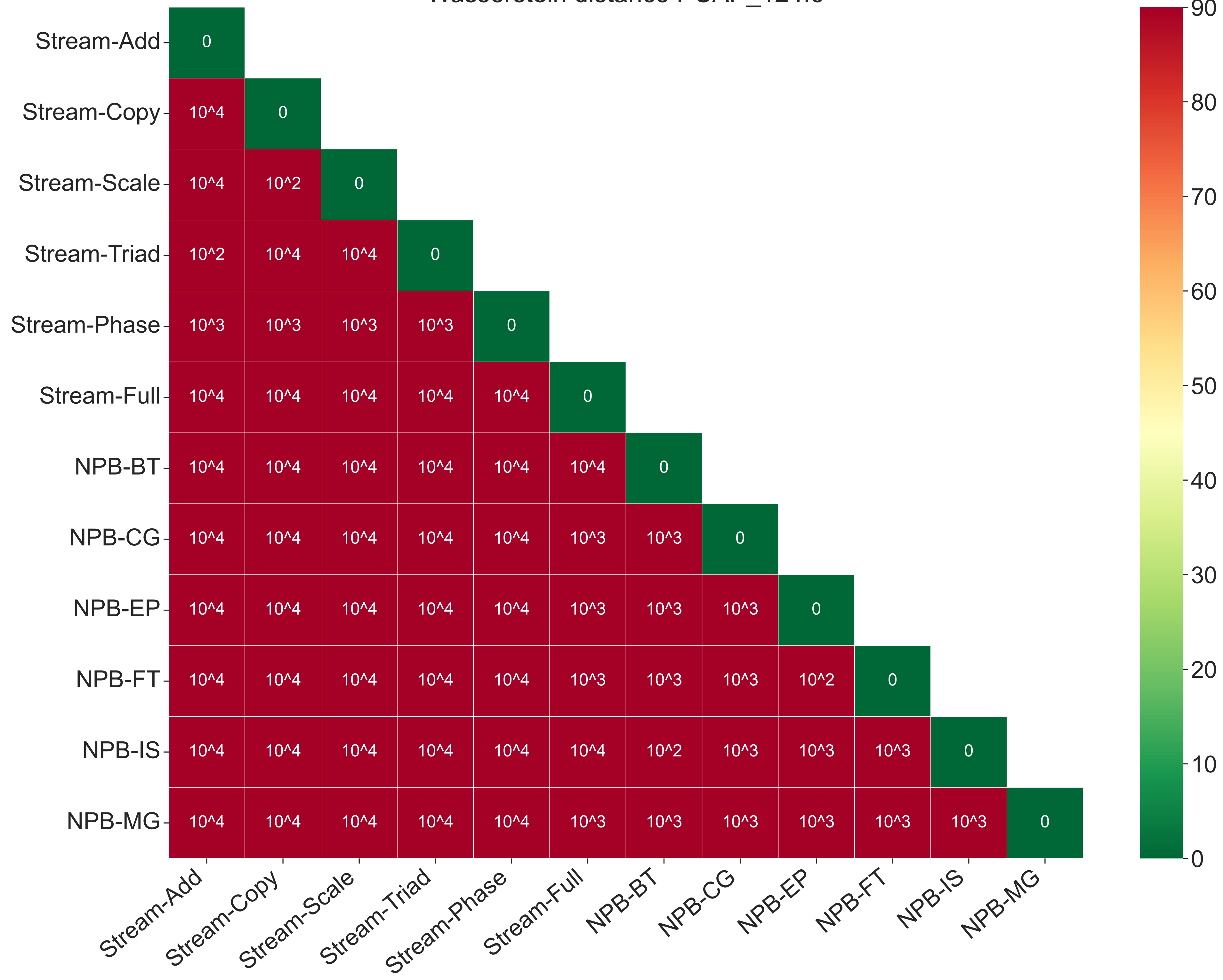
Wasserstein distance PCAP_124.0
