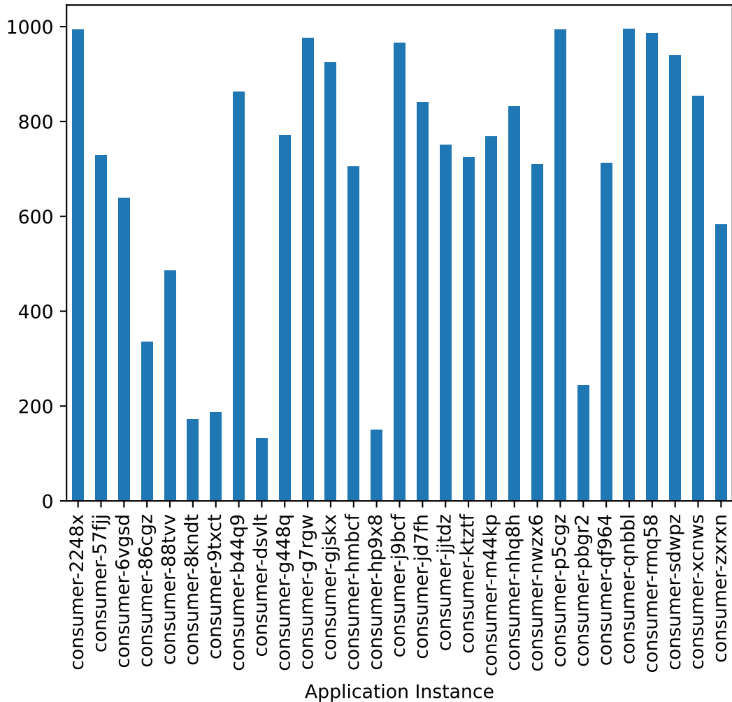
Averaged CPU Utilization (millicores)
