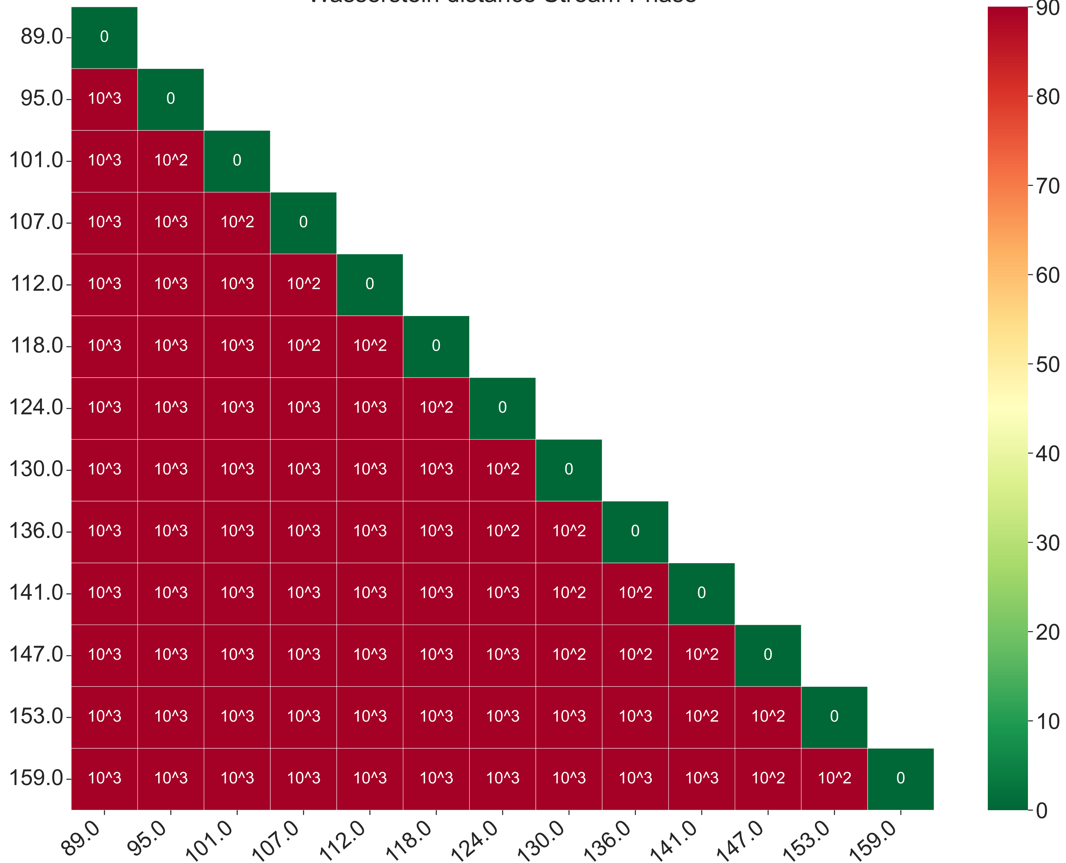
Wasserstein distance Stream-Phase
