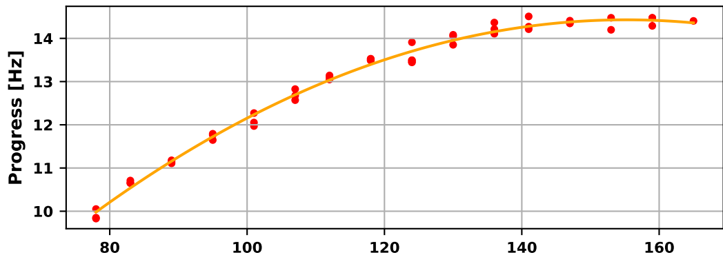
ones-npb-ep
