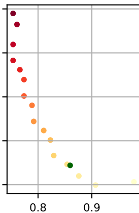
ones-stream-copy
