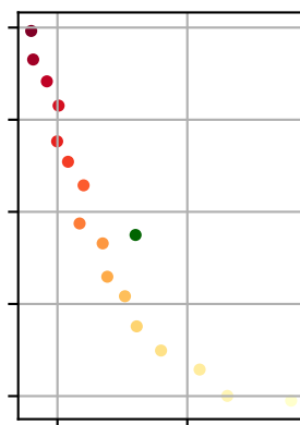
ones-npb-ep
