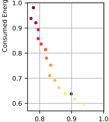
ones-stream-scale
