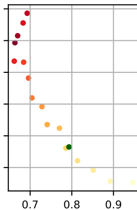
ones-npb-ep
