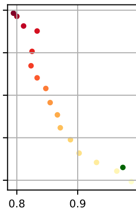
ones-stream-triad
