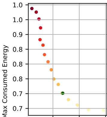
ones-stream-scale
