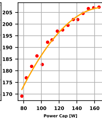
ones-stream-triad
