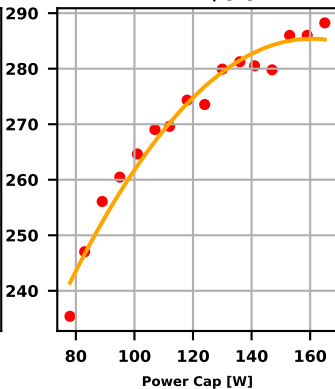
ones-stream-copy
