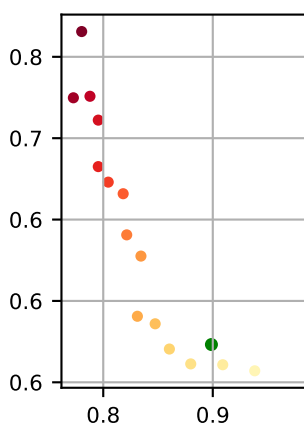
ones-stream-scale
