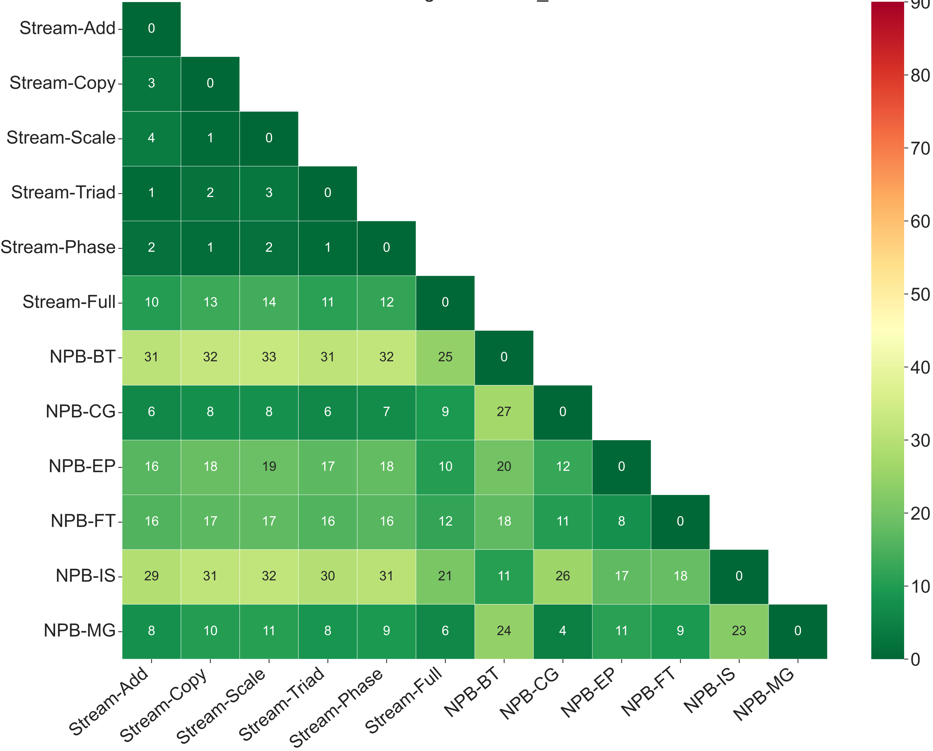
JS-divergence PCAP_124.0
