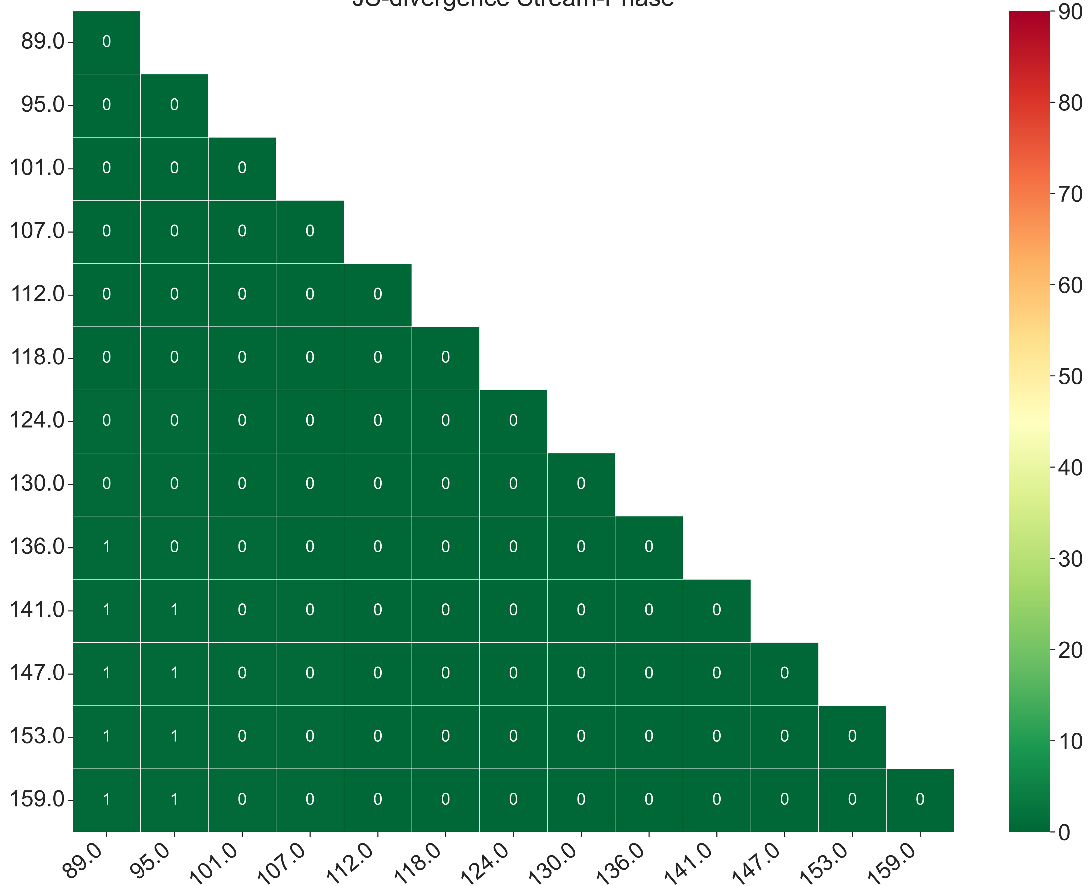
JS-divergence Stream-Phase
