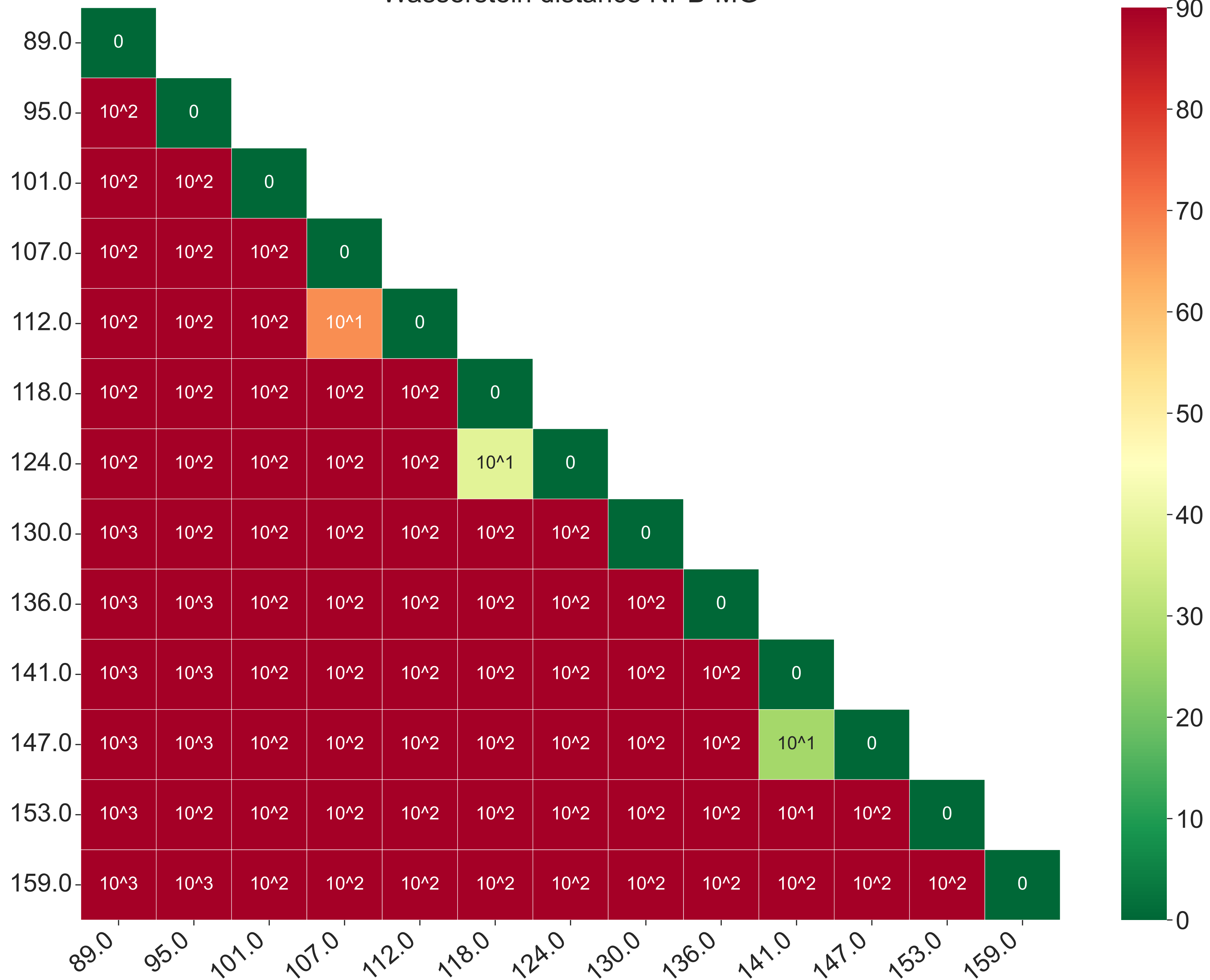
Wasserstein distance NPB-MG
