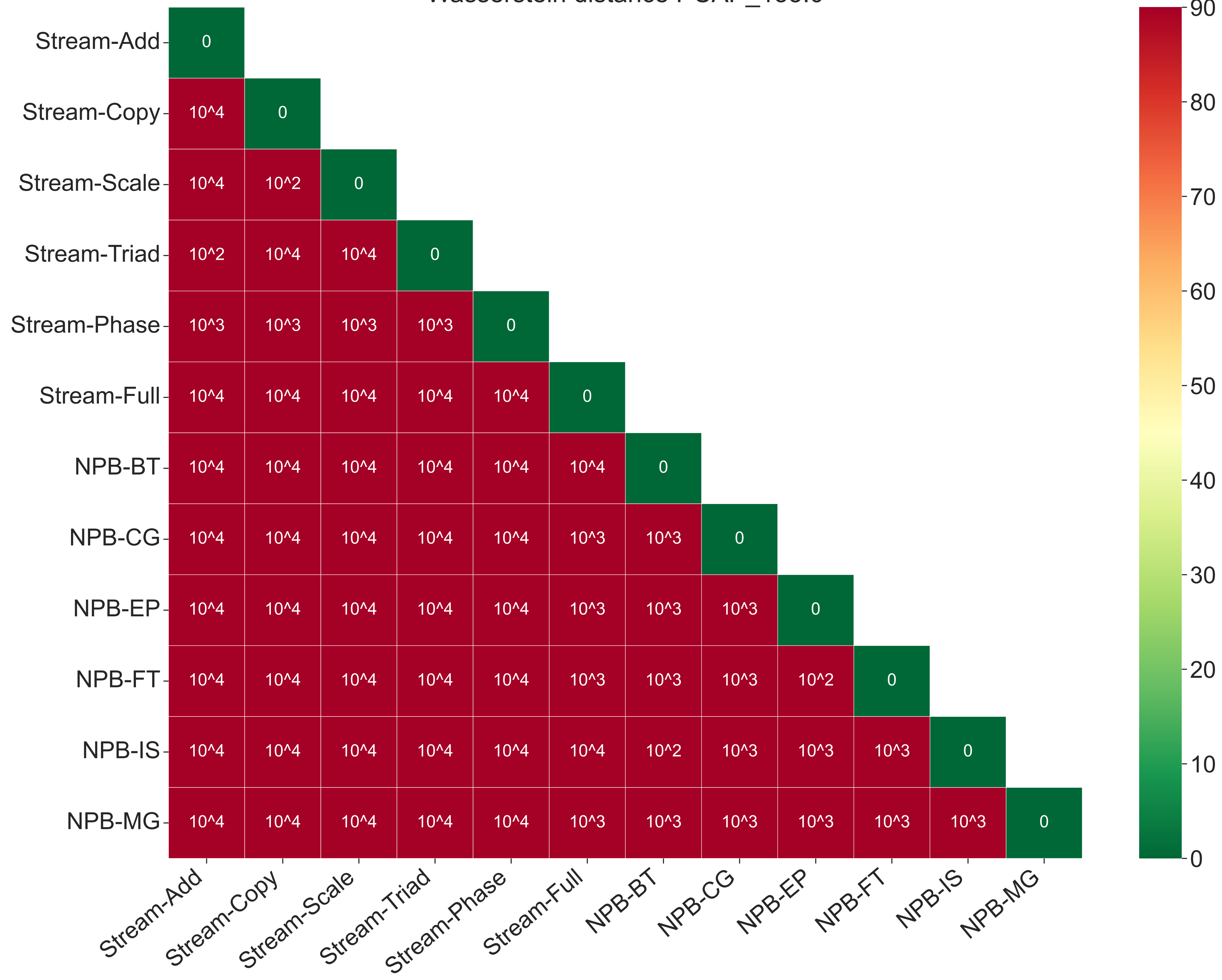
Wasserstein distance PCAP_153.0
