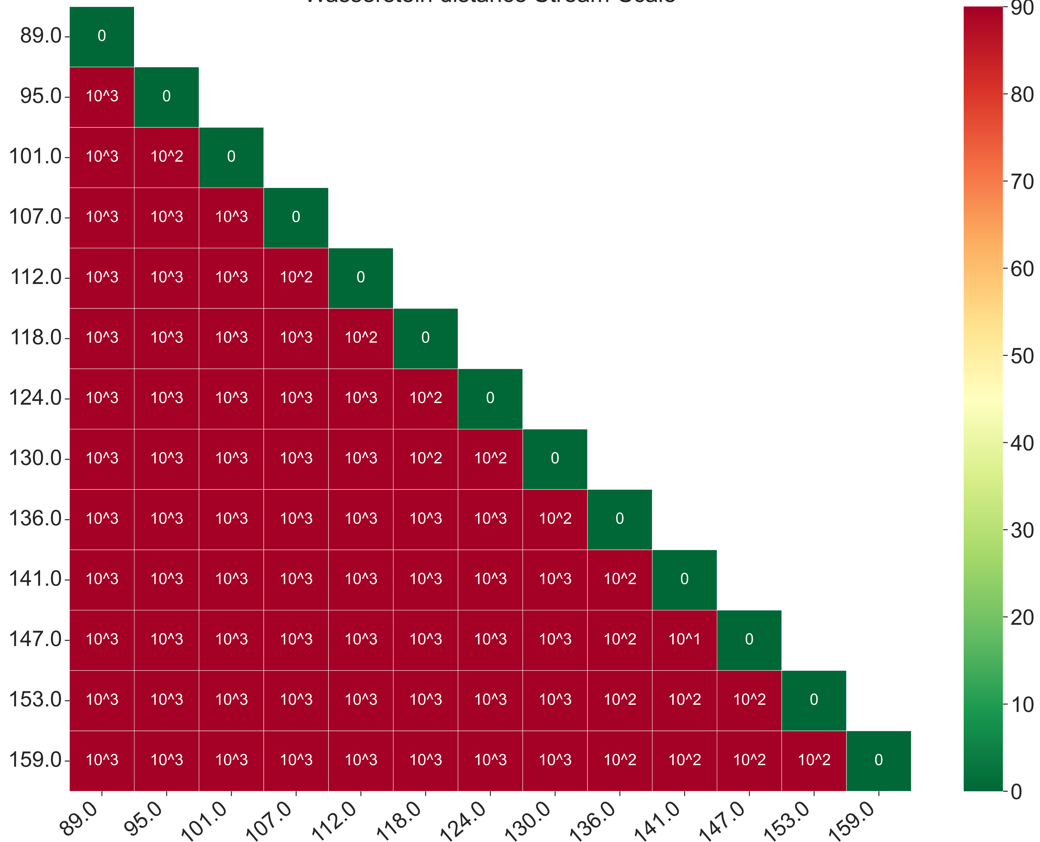
Wasserstein distance Stream-Scale
