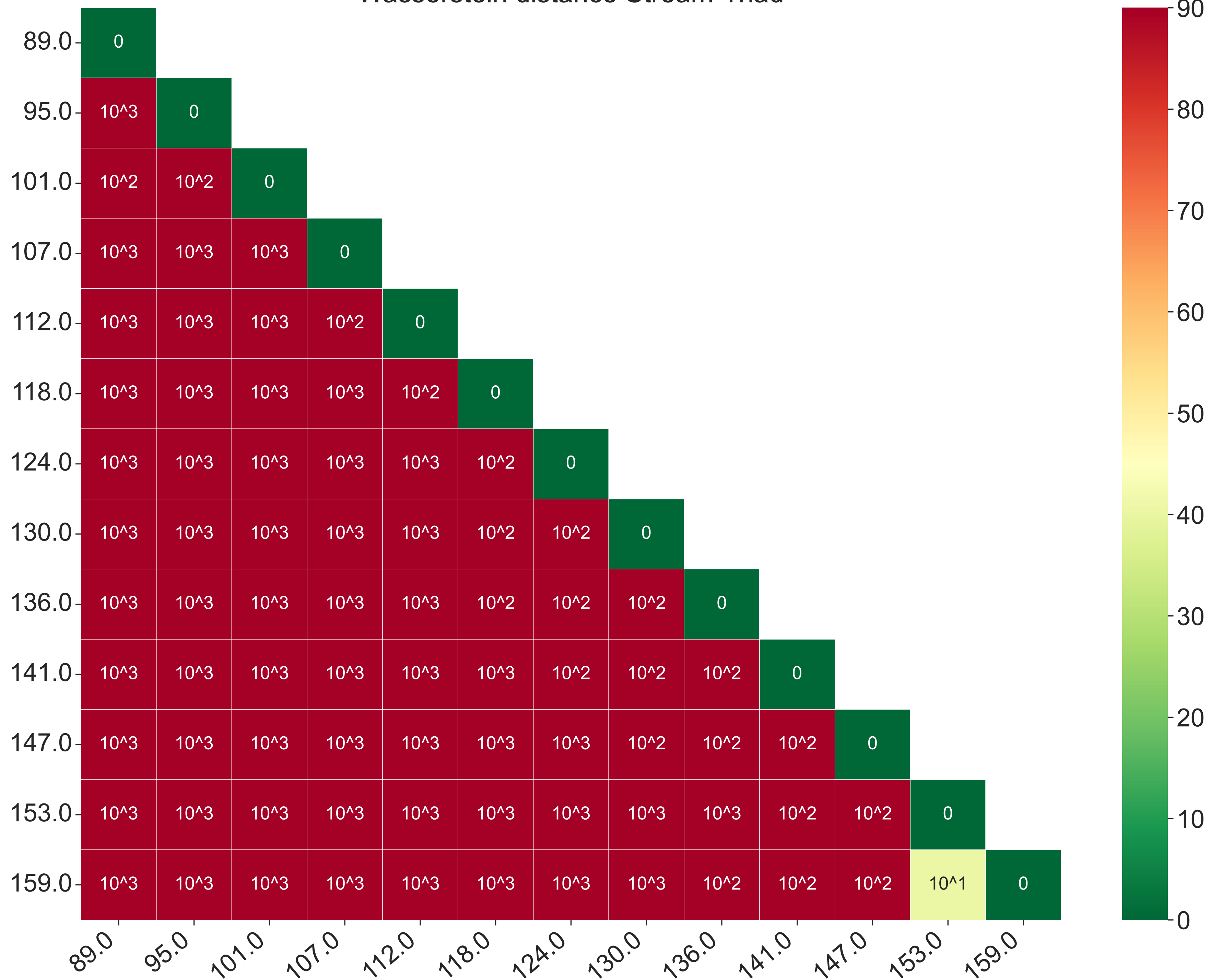
Wasserstein distance Stream-Triad
