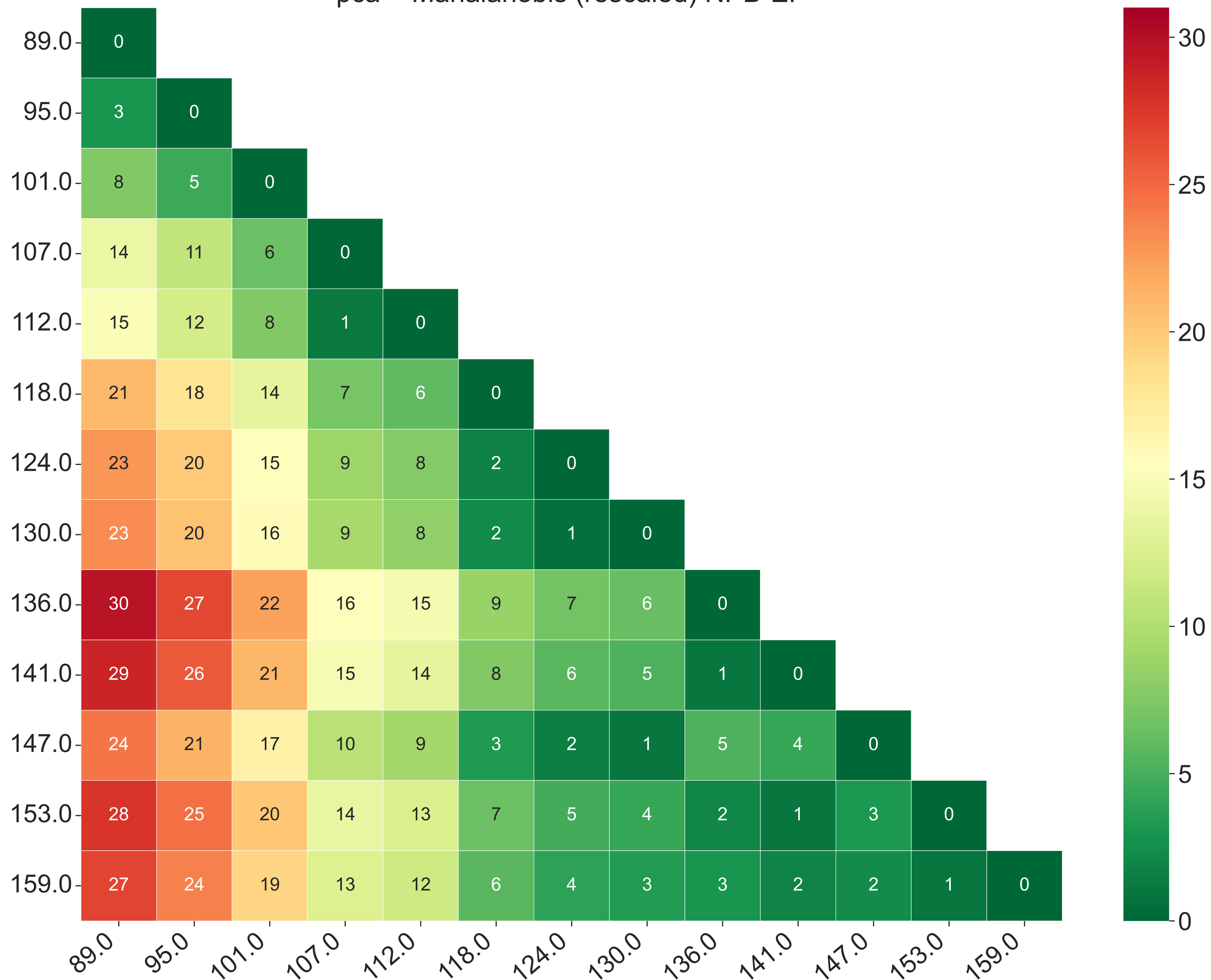
pca + Mahalanobis (rescaled) NPB-EP
