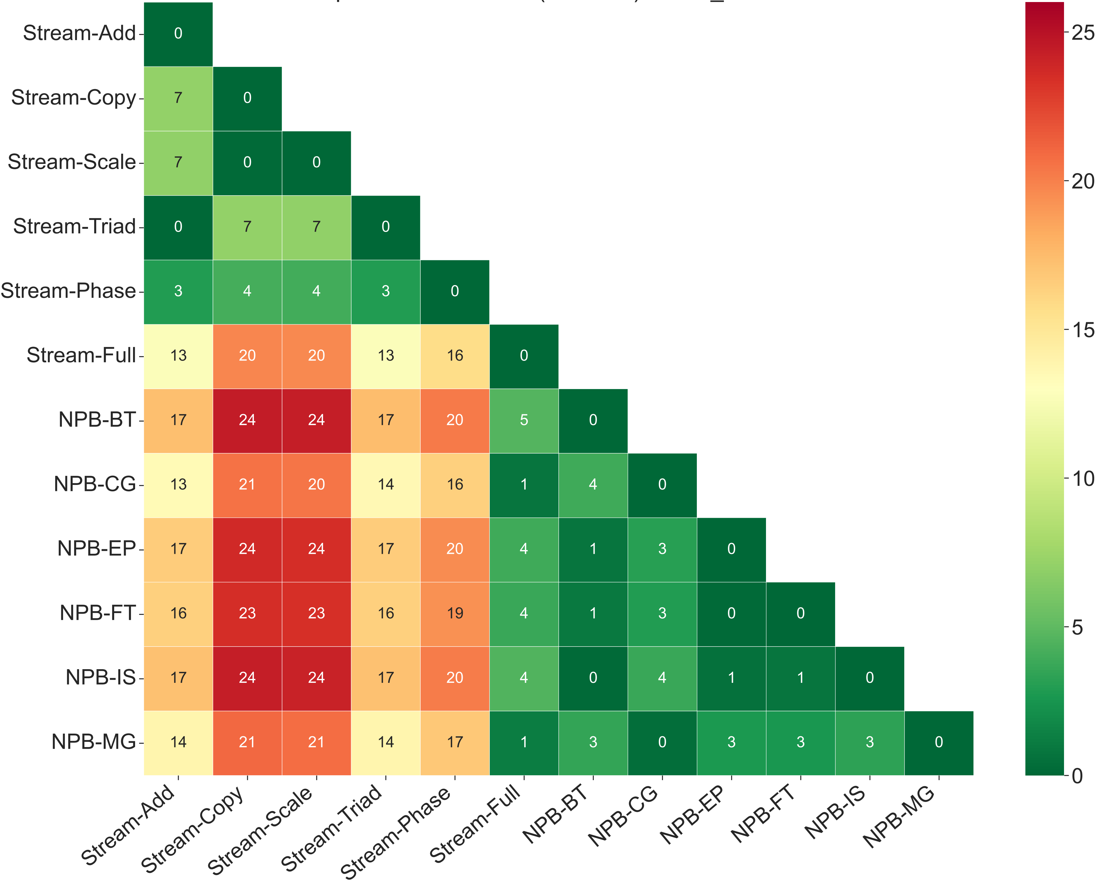
pca + Mahalanobis (rescaled) PCAP_124.0
