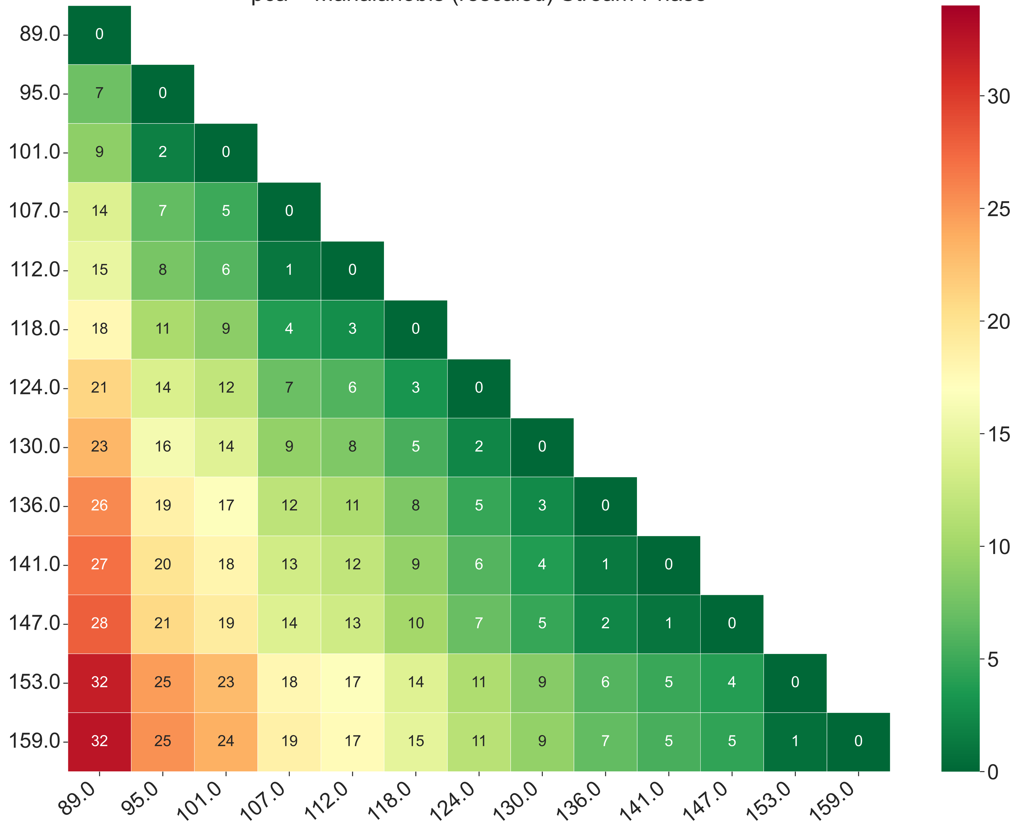
pca + Mahalanobis (rescaled) Stream-Phase
