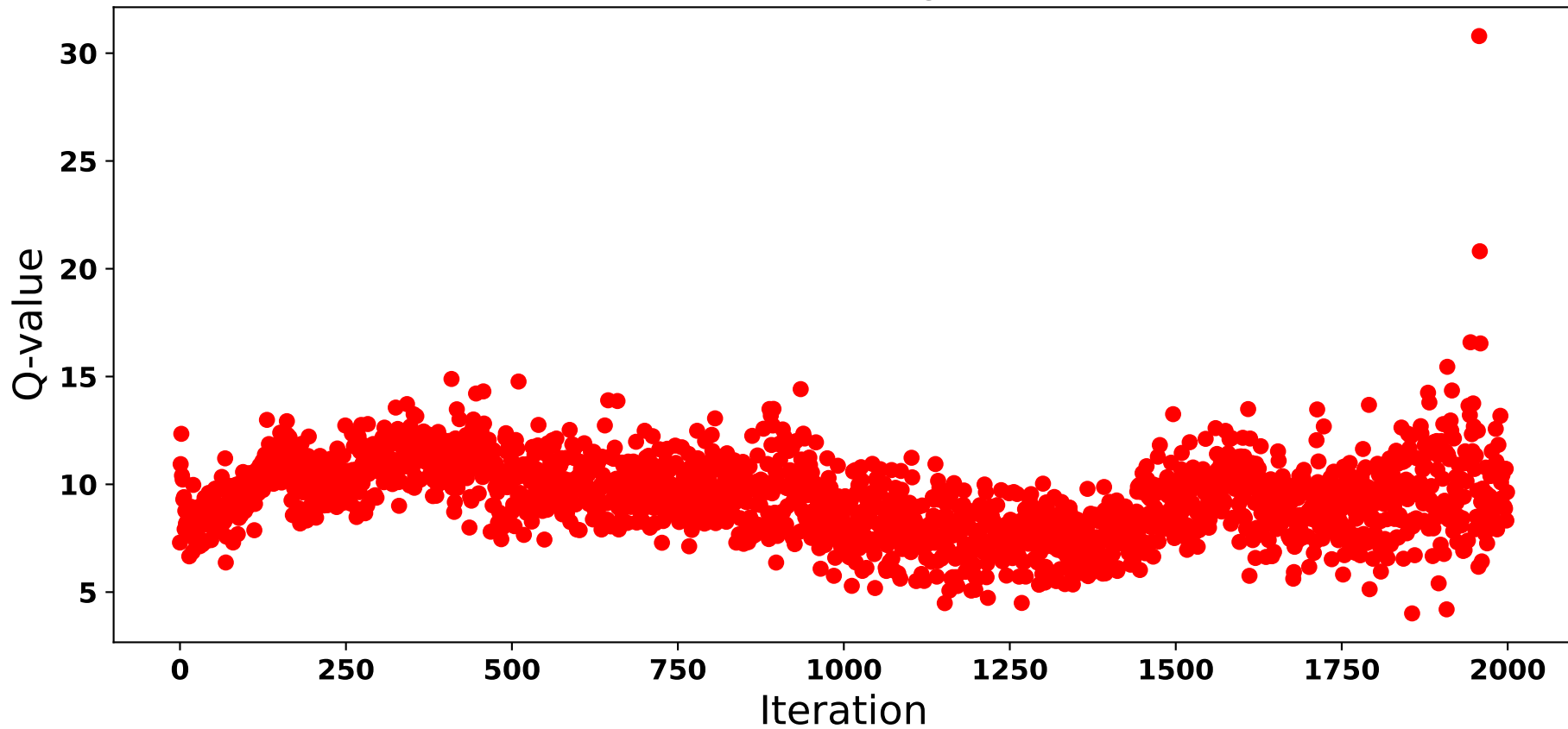
Q-value convergence
