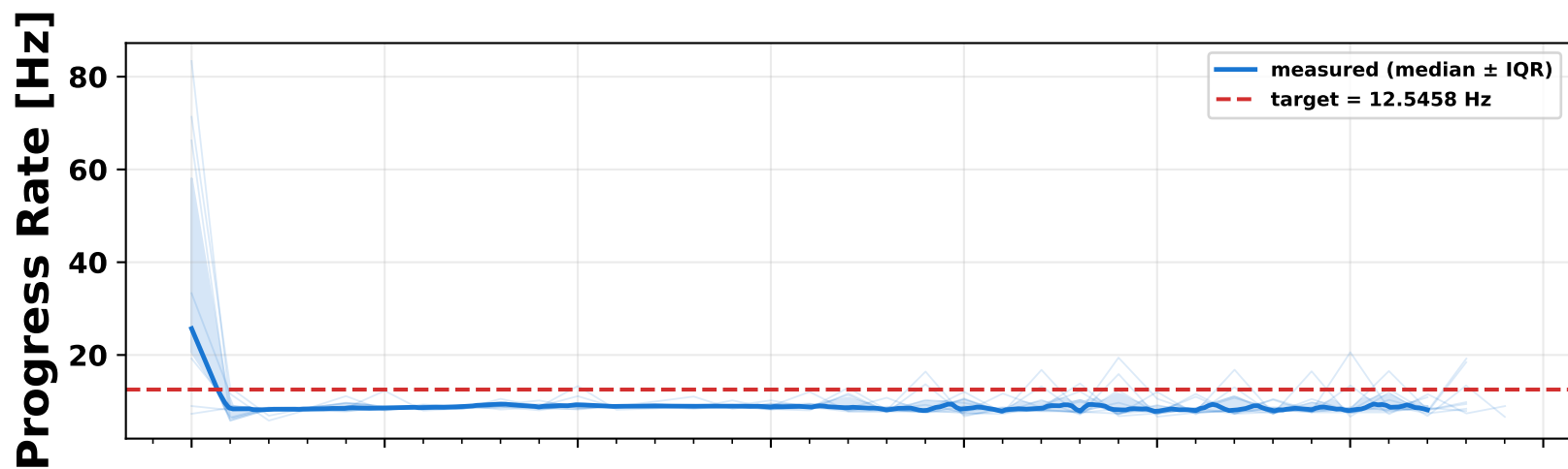
ones-npb-ft (10 iterations)
