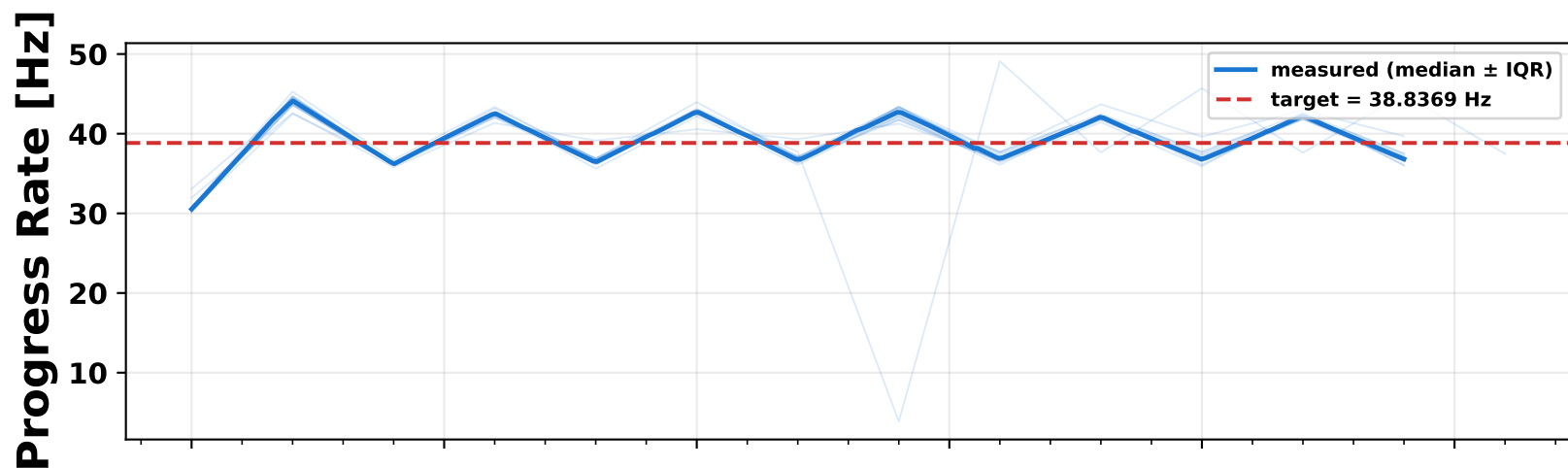
ones-npb-mg (10 iterations)
