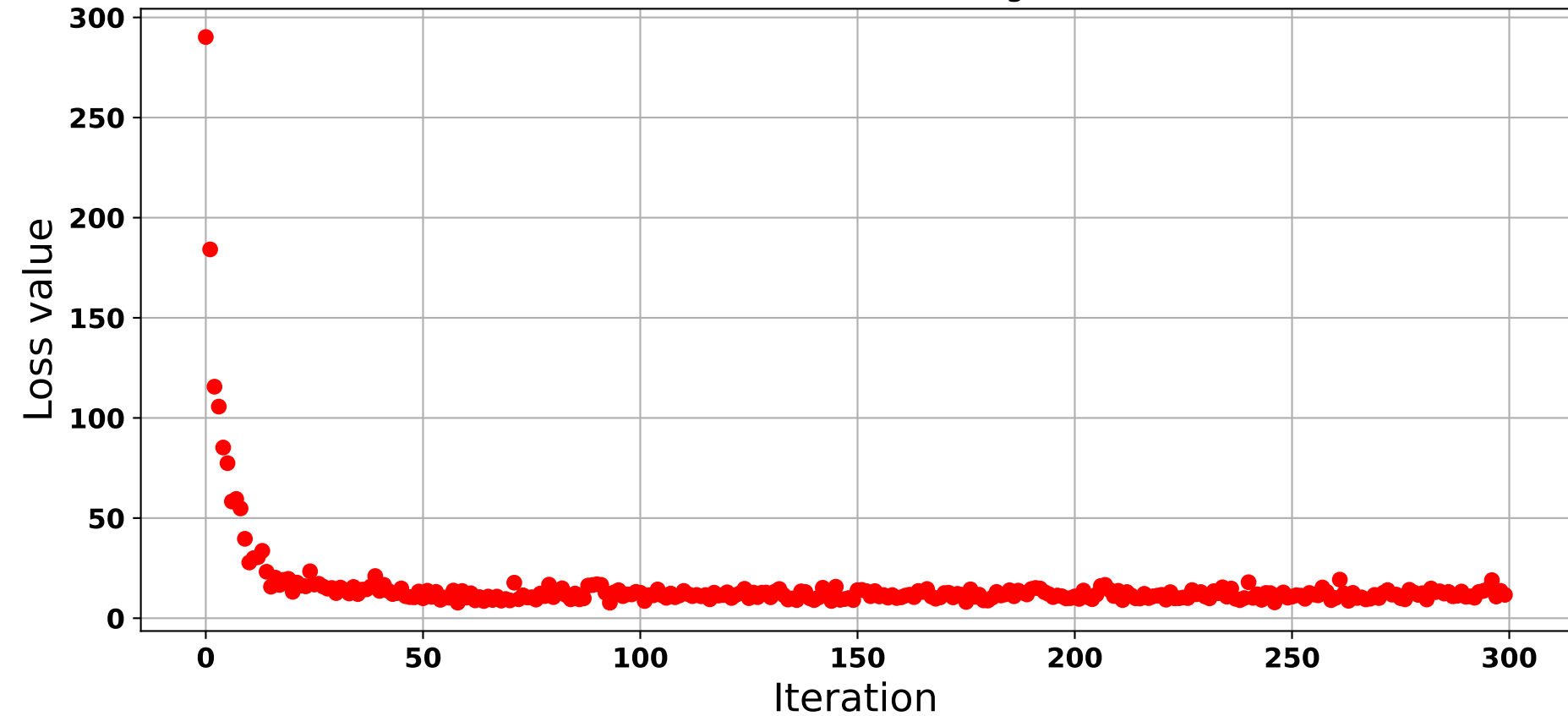
RL actor network convergence
