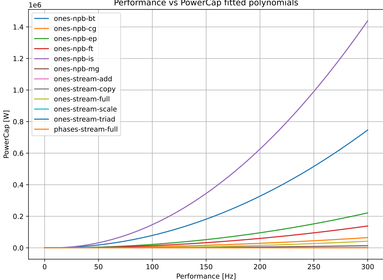
Performance vs PowerCap fitted polynomials
