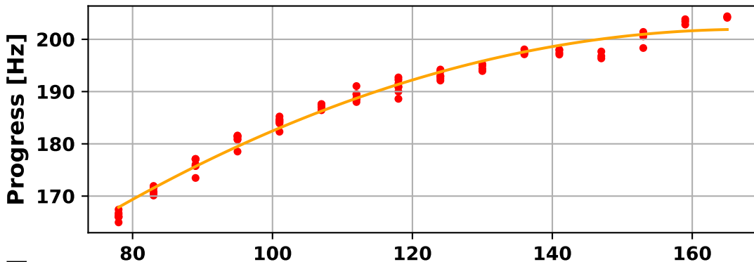
ones-stream-triad
